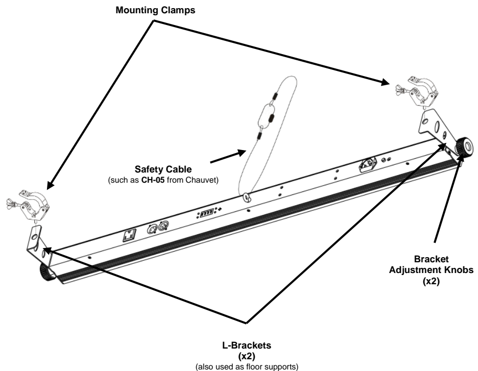
Mounting Diagram
